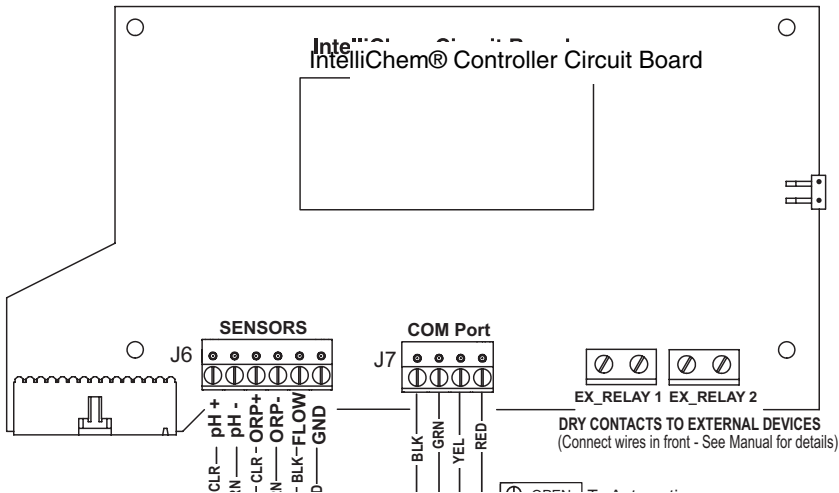
Figure 2: IntelliChem® Controller J6/J7 Circuit Board Wiring
