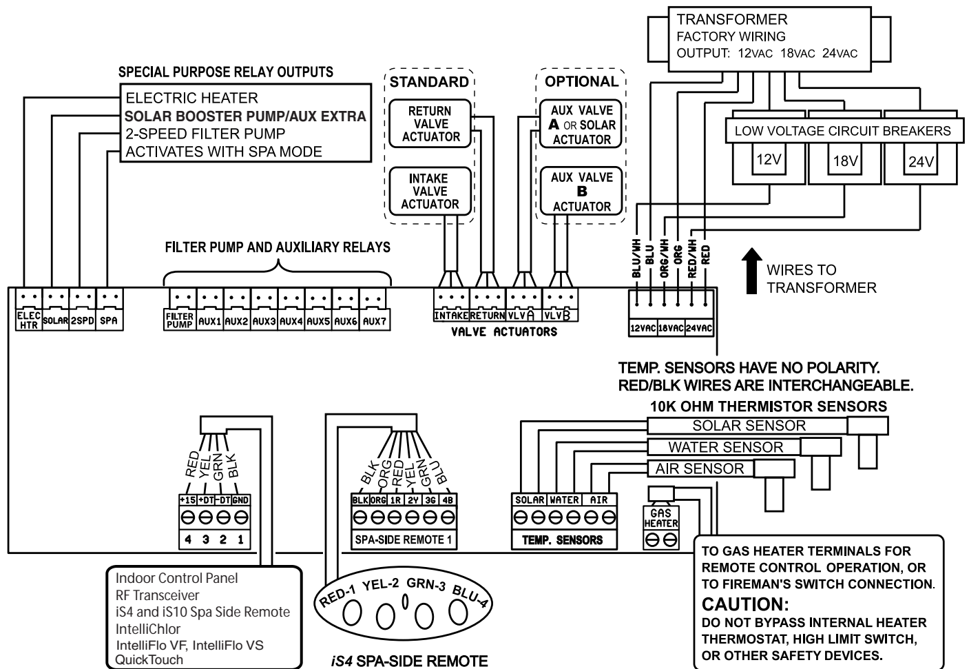
EasyTouch System Wiring Diagram (Outdoor Control Panel)
