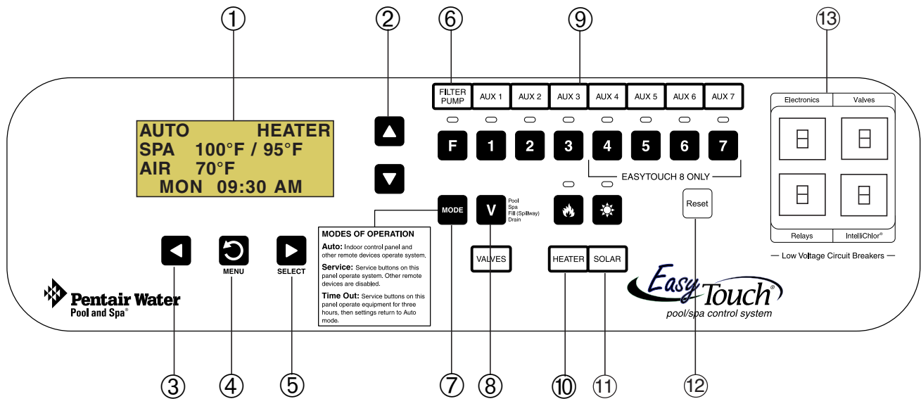
EasyTouch 8 Outdoor Control Panel
